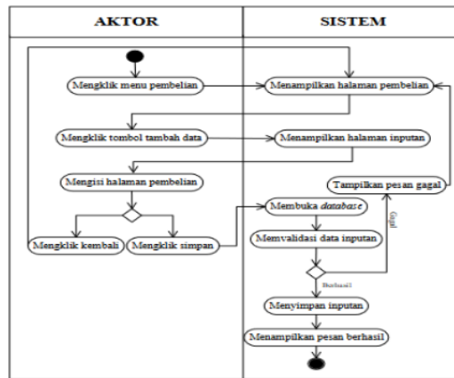
Gambar 3. Activity Diagram Pembelian
