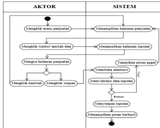
Gambar 4. Activity Diagram Penjualan
